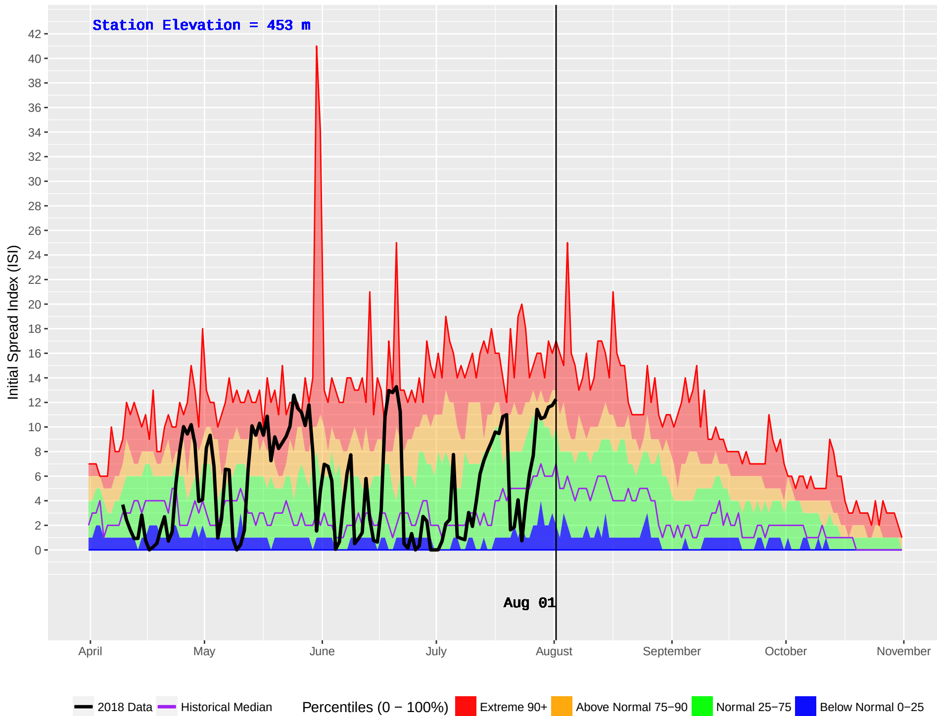
CLEARWATER HUB (239) : Historical (1976–2016) and Current (2018) Daily Initial Spread Index (ISI)
