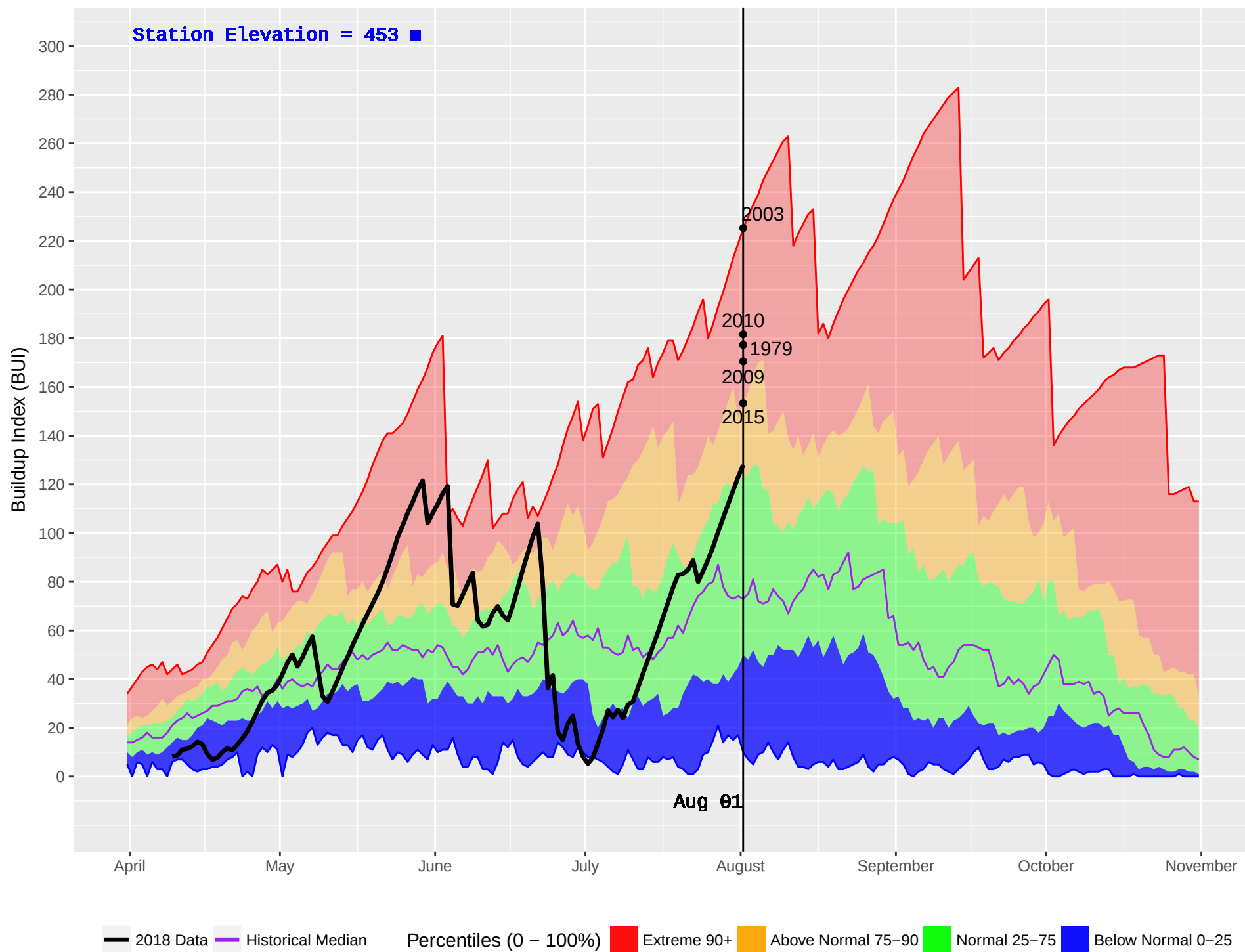
CLEARWATER HUB (239) : Historical (1976–2016) and Current (2018) Daily Buildup Index (BUI)
