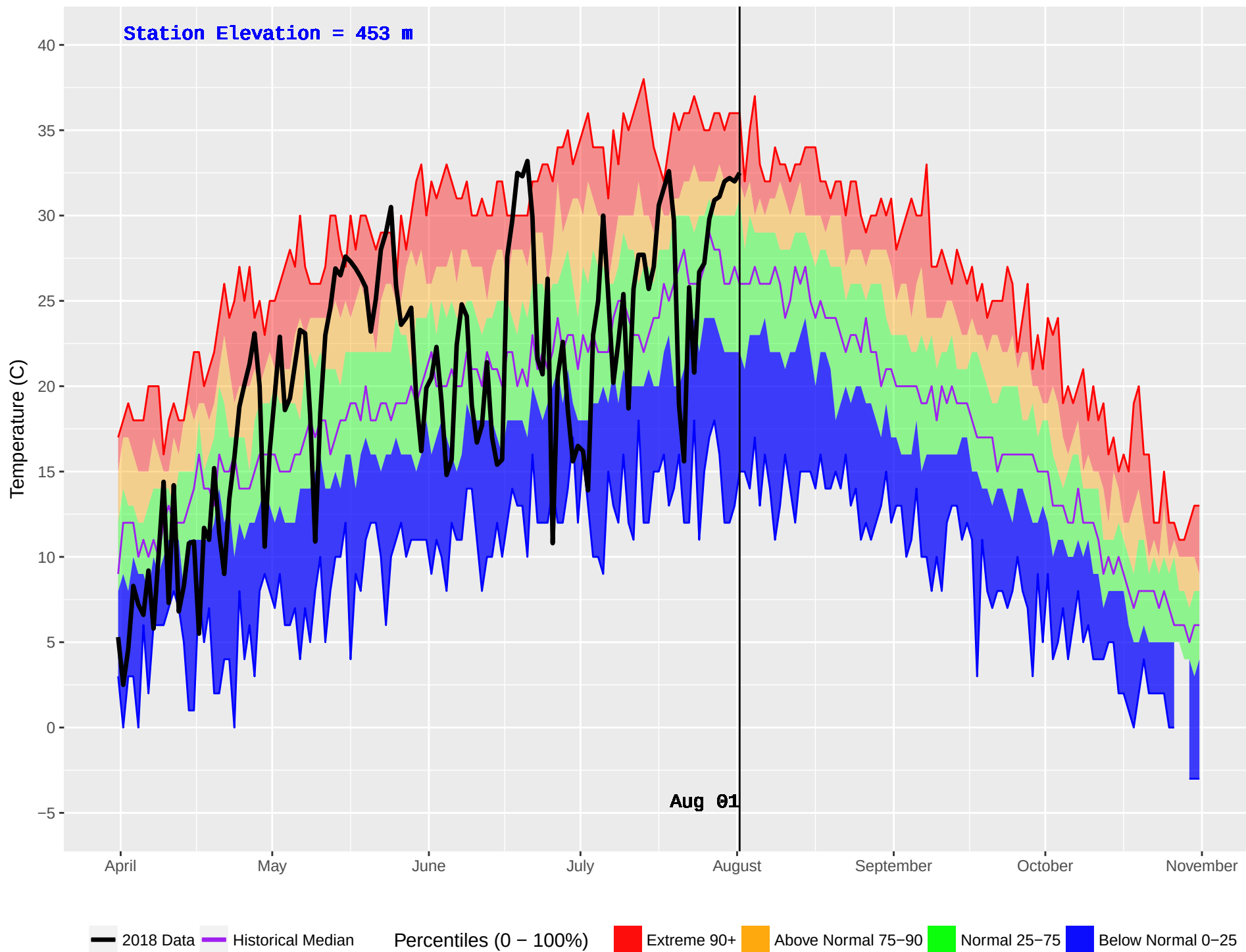
CLEARWATER HUB (239) : Historical (1976–2016) and Current (2018) Daily Temperature
