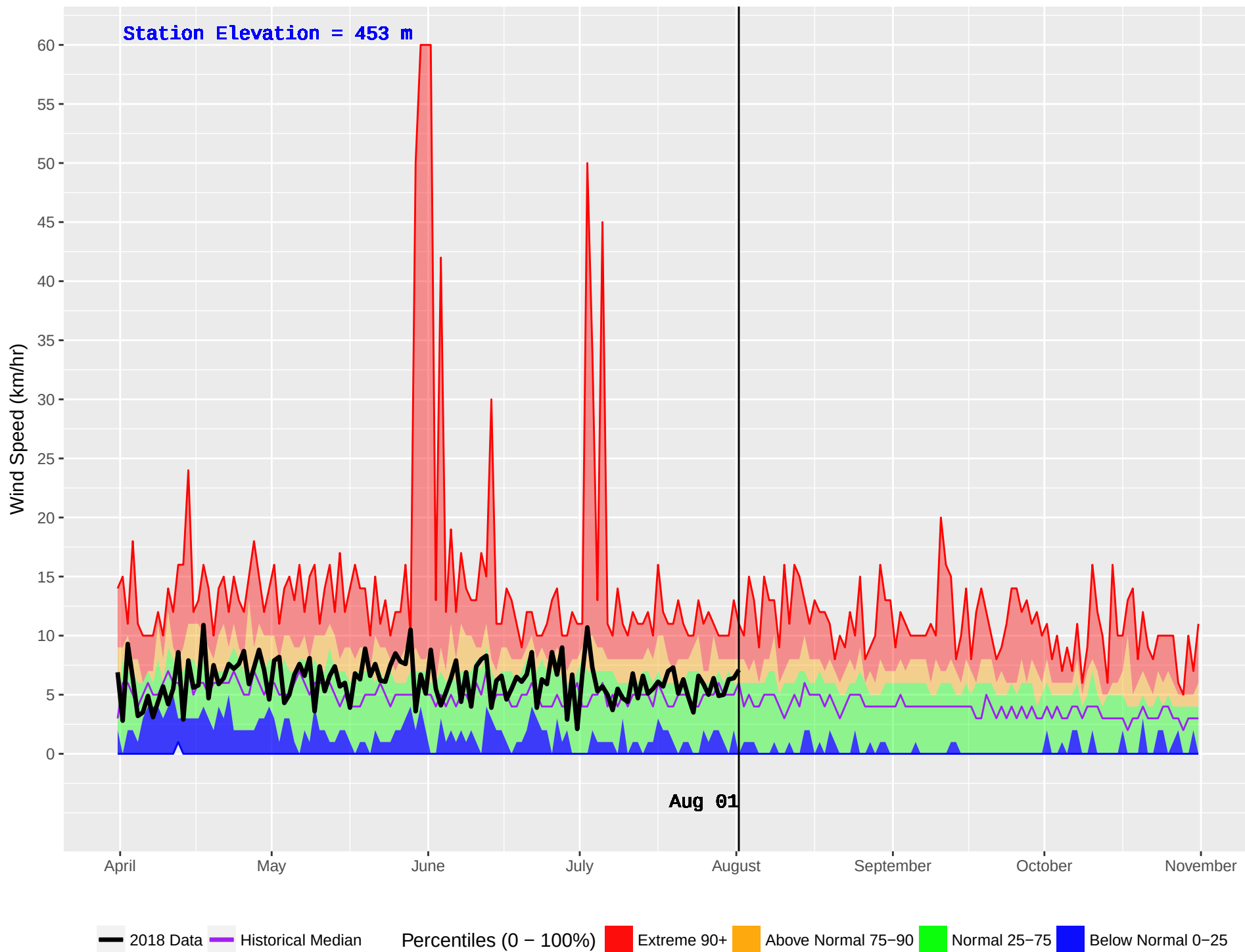
CLEARWATER HUB (239) : Historical (1976–2016) and Current (2018) Daily Wind Speed
