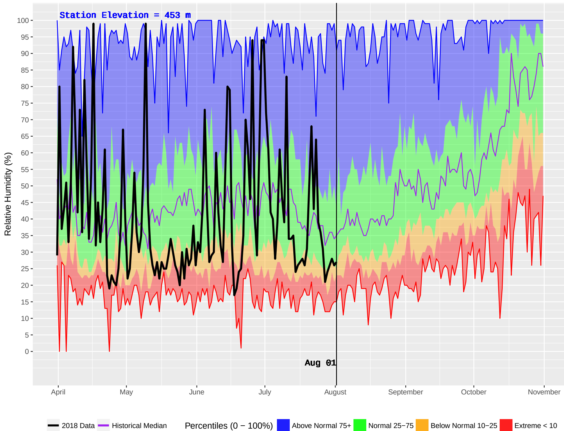
CLEARWATER HUB (239) : Historical (1976–2016) and Current (2018) Daily Relative Humidity
